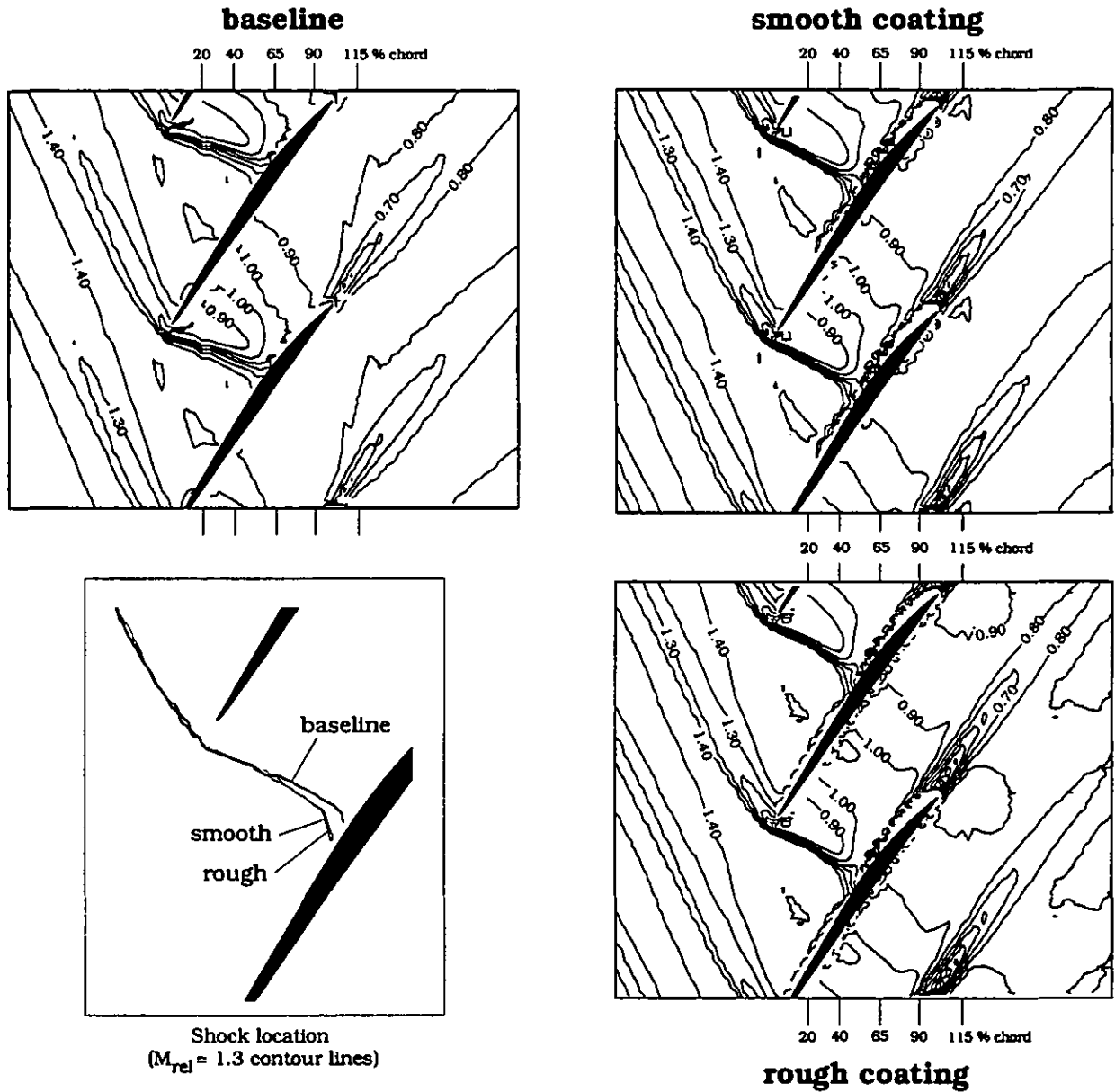
FIGURE 13. LASER ANEMOMETER MEASUREMENTS OF RELATIVE MACH NUMBER ON THE 70% SPAN STREAMSURFACE
