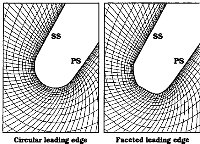
FIGURE 16. CFD GRID DETAIL AT THE LEADING EDGE
