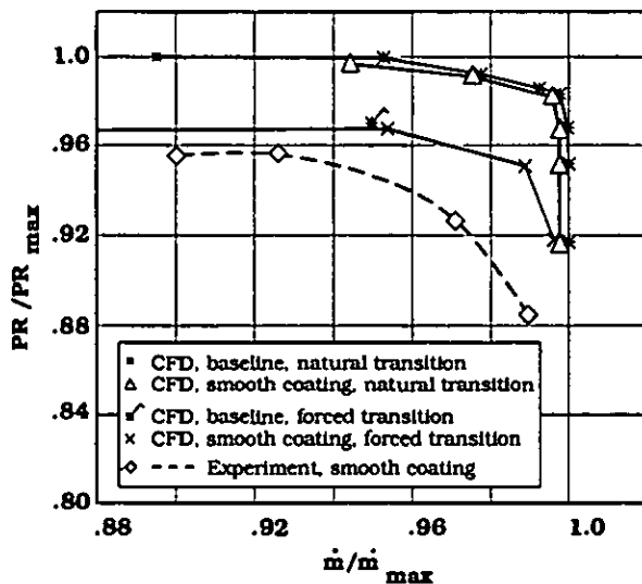
FIGURE 17. COMPARISON BETWEEN PREDICTED AND MEASURED PRESSURE RISE VS MASSFLOW CHARACTERISTICS AT 70% SPAN FOR THE ROUGH-COATED BLADE
