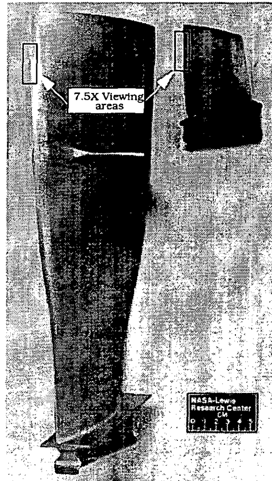
FIGURE 1a. COMPARISON BETWEEN ENGINE FAN BLADE AND THE RESEARCH ROTOR BLADE
