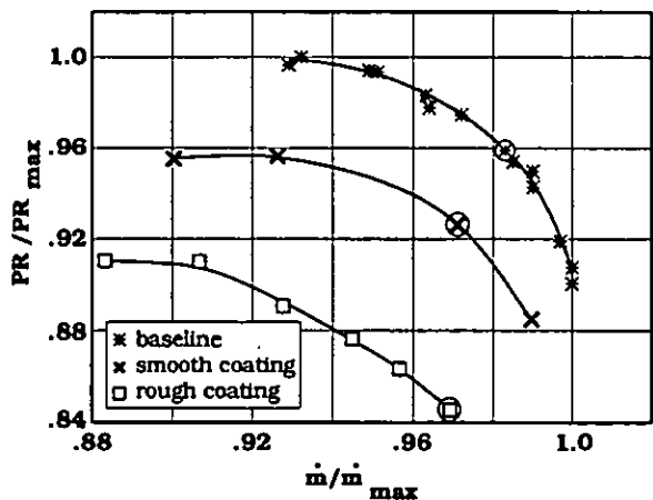
FIGURE 11. PRESSURE RATIO VS MASSFLOW CHARACTERISTICS AT 70% SPAN. CIRCLED POINTS INDICATE OPERATING CONDITIONS DURING LASER ANEMOMETER SURVEYS
