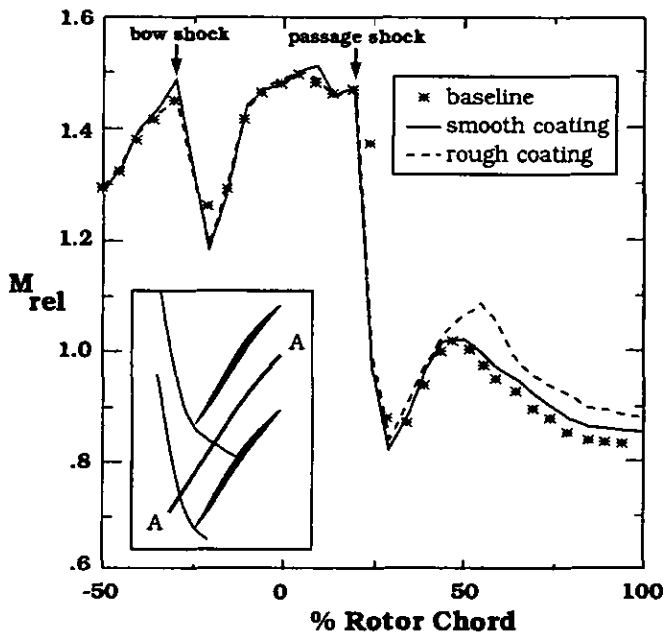
FIGURE 14. LASER ANEMOMETER MEASUREMENTS OF RELATIVE MACH NUMBER ALONG THE MID-PITCH LINE, A-A, AT 70% SPAN
