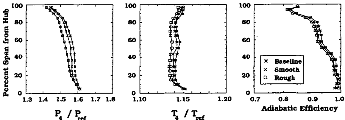
(B) 80% SPEED, NEAR PEAK EFFICIENCY, 17.44 KG/S
