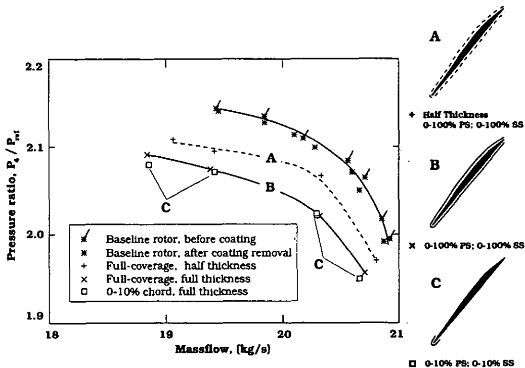
FIGURE 8. PRESSURE RISE CHARACTERISTICS FOR THE SMOOTH COATINGS AT DESIGN SPEED
