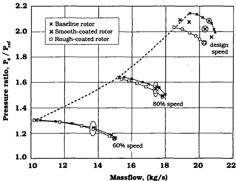
FIGURE 4. PRESSURE RISE CHARACTERISTICS FOR FULL- COVERAGE COATINGS. CIRCLED POINTS INDICATE OPERATING CONDITIONS FOR WHICH RADIAL DISTRIBUTIONS OF FLOW PROPERTIES ARE PRESENTED
