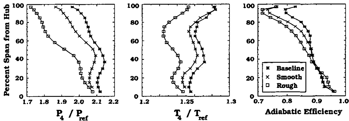
(A) 100% SPEED, NEAR PEAK EFFICIENCY, 20.31 KG/S
