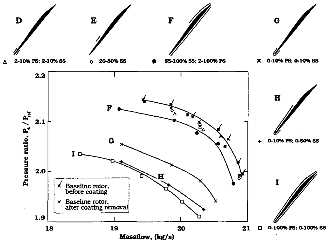
FIGURE 9. PRESSURE RISE CHARACTERISTICS FOR THE ROUGH COATINGS AT DESIGN SPEED
