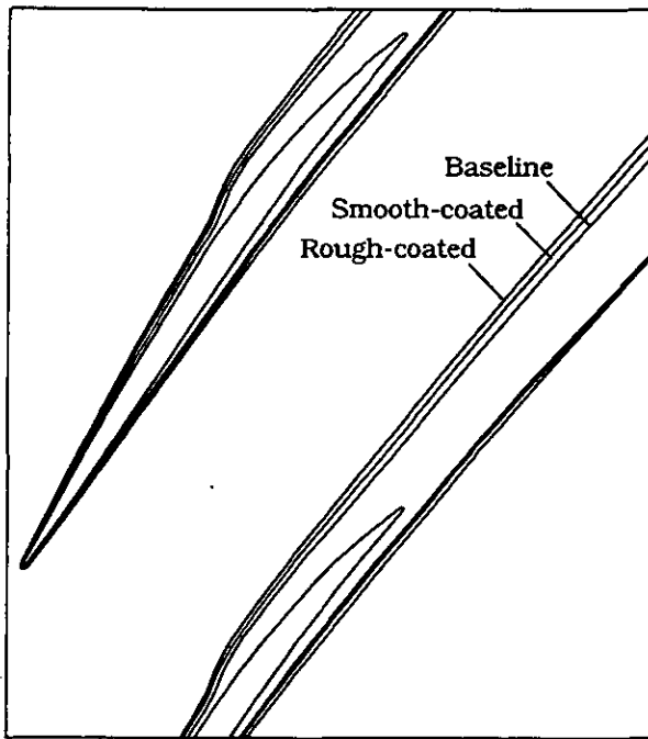
FIGURE 19. PREDICTED BOUNDARY LAYER GROWTH VISUALIZED AS A LOCUS OF CONSTANT ENTROPY
