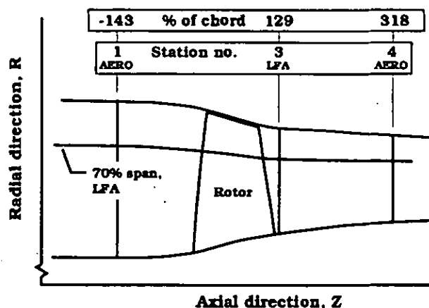
FIGURE 2. LASER ANEMOMETER AND AERODYNAMIC SURVEY STATIONS
