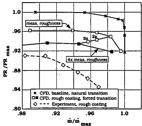
FIGURE 18. COMPARISON BETWEEN PREDICTED AND MEASURED PRESSURE RISE VS MASSFLOW CHARACTERISTICS AT 70% SPAN FOR THE ROUGH-COATED BLADE
